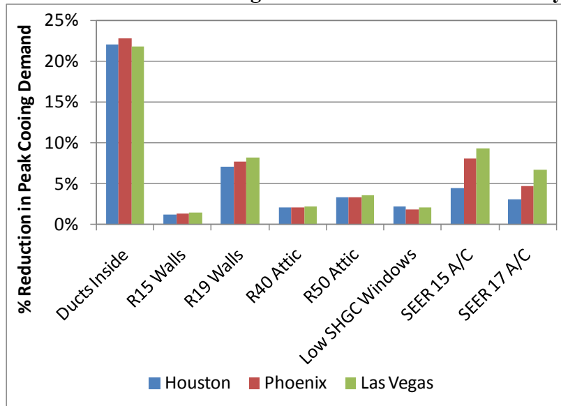
Figure 6. Reduction in Peak Cooling Demand for Various Efficiency Upgrades
